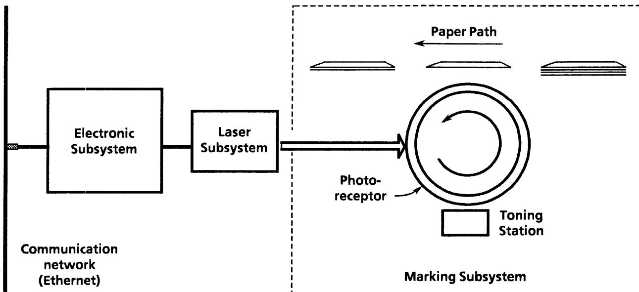
Figure 10-1 Electronic printing
