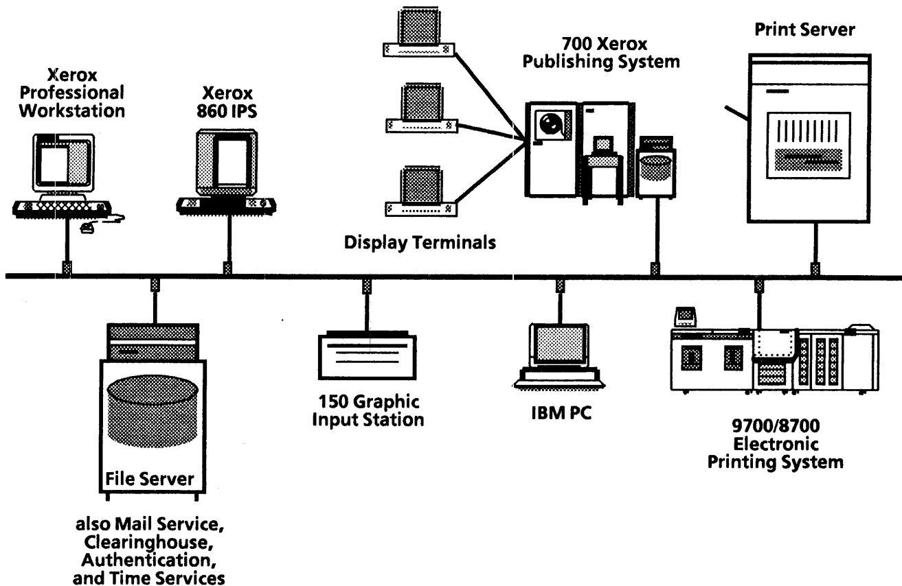
Figure 12-7 Electronic publishing using the 700 Xerox Publishing System
