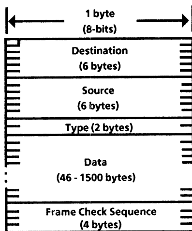
Figure 3-2 Ethernet frame
