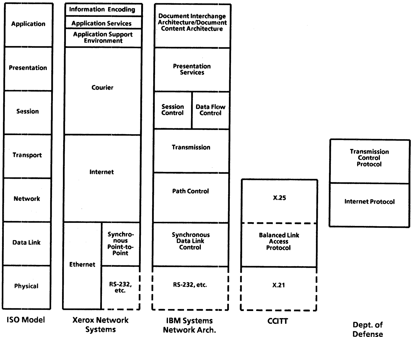
Figure B-1 XNS and other architectures
