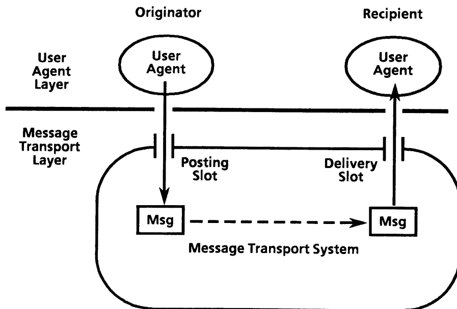
Figure 9-1 CCITT X.400 architecture model
